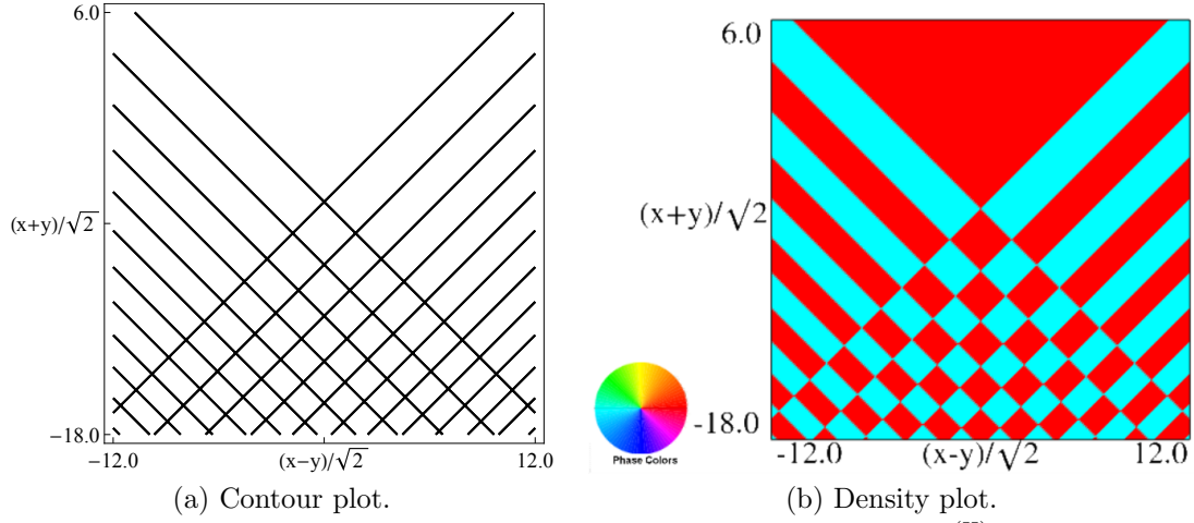
Figure 36.3.18: Phase of hyperbolic umbilic canonical integral \text{ph } \Psi^{(\text{H})}(x, y, 0) .
