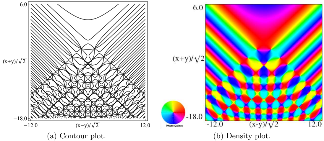
Figure 36.3.19: Phase of hyperbolic umbilic canonical integral \text{ph } \Psi^{(\text{H})}(x, y, 1) .
