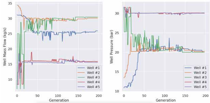
Results from an AI experiment using genetic algorithms to optimize generation by varying mass flow and well pressure. Figure by National Laboratory of the Rockies
