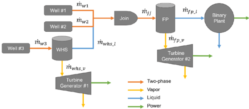
Semantic model architecture illustrating GOOML's modular approach to developing configurable digital twins for geothermal plants. Figure by Upflow, Ltd. and NLR.
