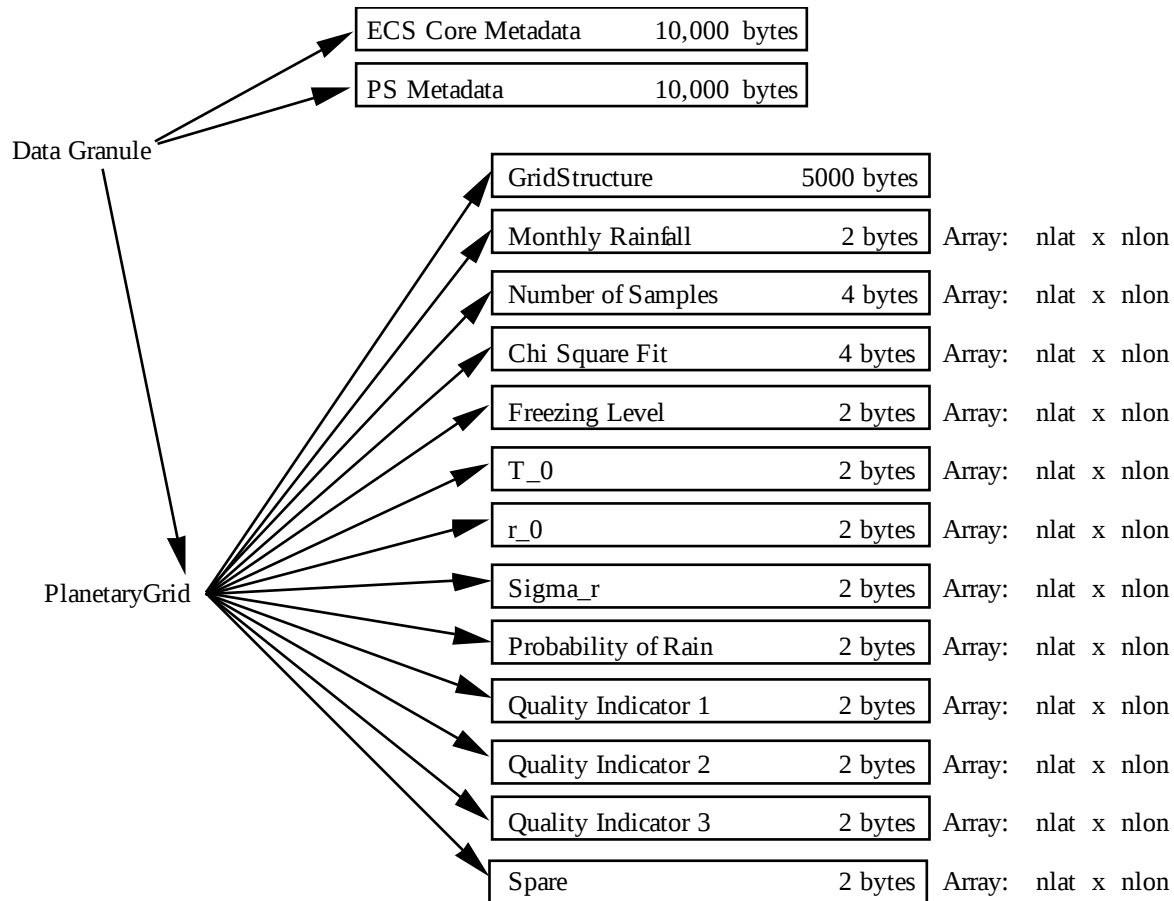
Figure 2.1.1-1 Data Format Structure for 3A-11, TMI Emission
