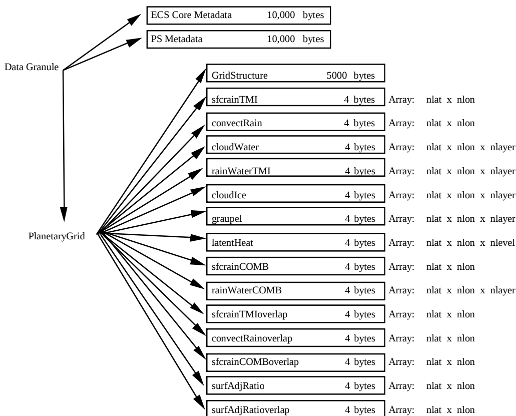
Figure 2.3.1-1 Data Format Structure for 3B-31, Rainfall Combined.
