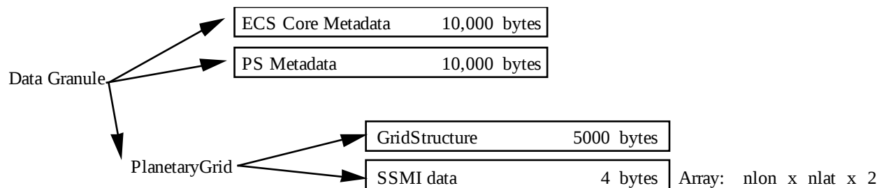
Figure 2.6.1-1 Data Format Structure for 3A-46, SSM/I Rain.
