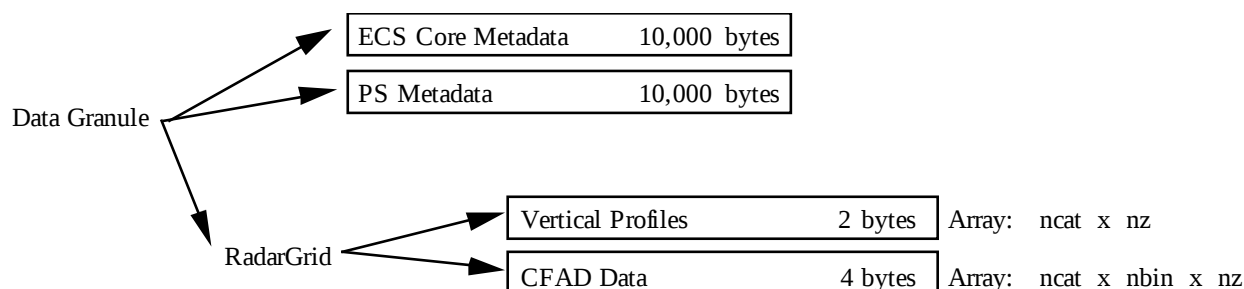
Figure 2.5.3-1 Data Format Structure for 3A-55, Monthly 3-D Structure (Previous Page).
