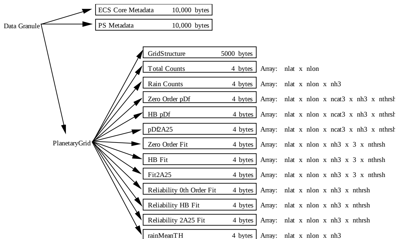
Figure 2.2.2-1 Data Format Structure for 3A-26, Surface Rainfall.
