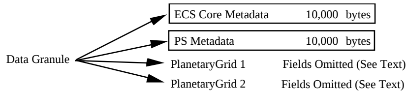
Figure 2.2.1-1 Data Format Structure for 3A-25, PR Rainfall
